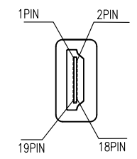
Conn.2 HDMI Female
